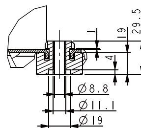
Foot Base
